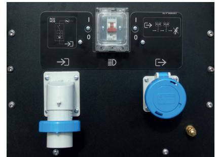
Standard control panel
